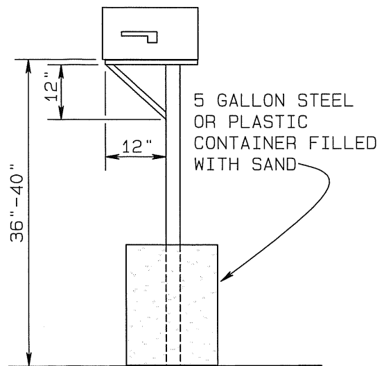
TEMPORARY INSTALLATION
