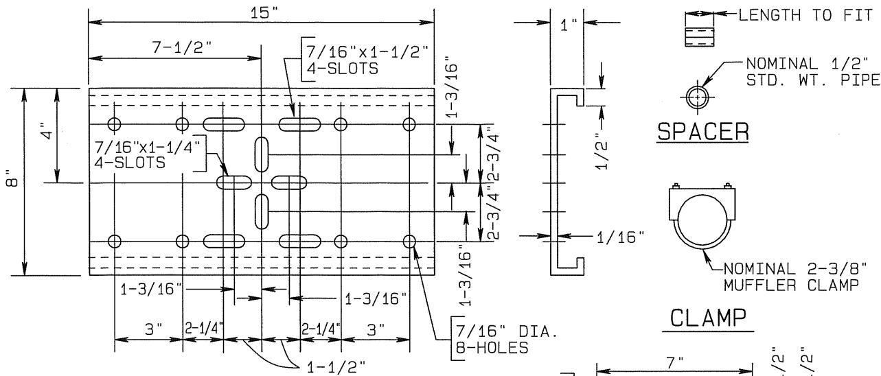
SHELF
