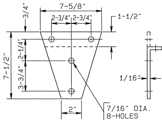
BRACKET
