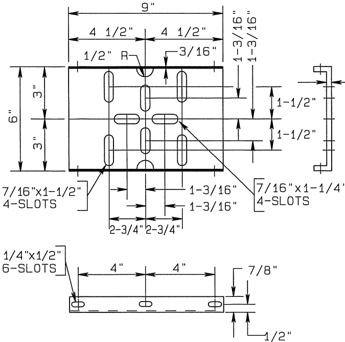
PLATFORM
