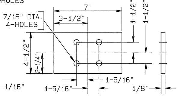
ANTI-TWIST PLATE
