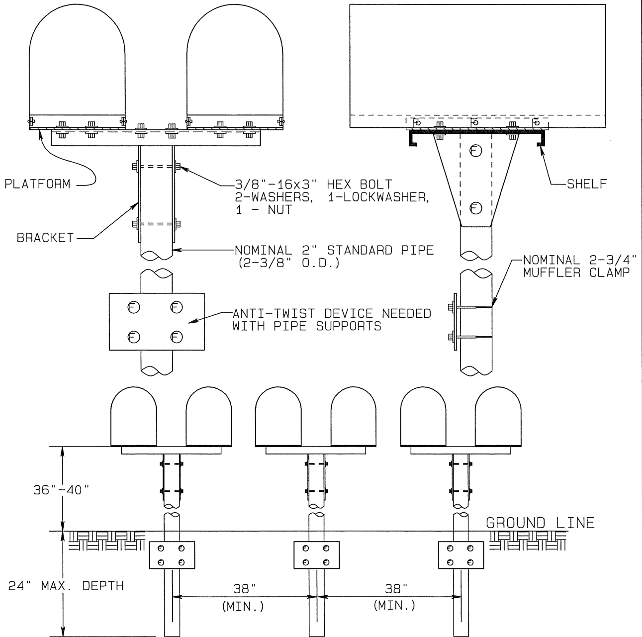
SPACING FOR MULTIPLE POST INSTALLATION
