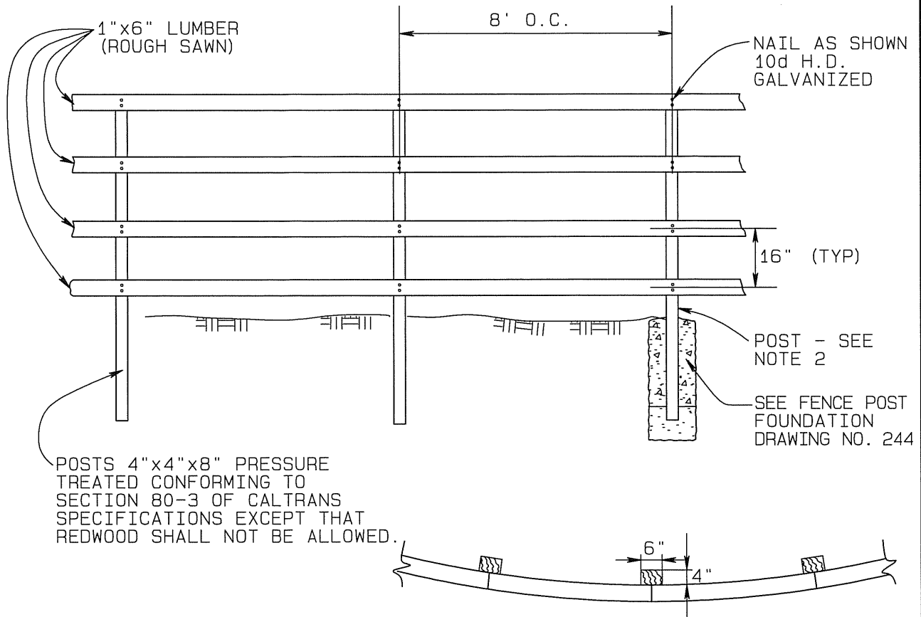
PLAN VIEW FOR FENCE ALONG HORIZONTAL CURVE
