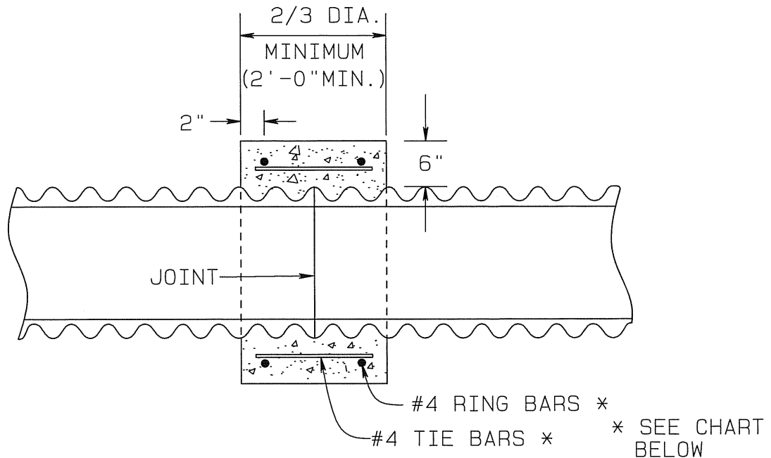
COLLAR DETAIL
