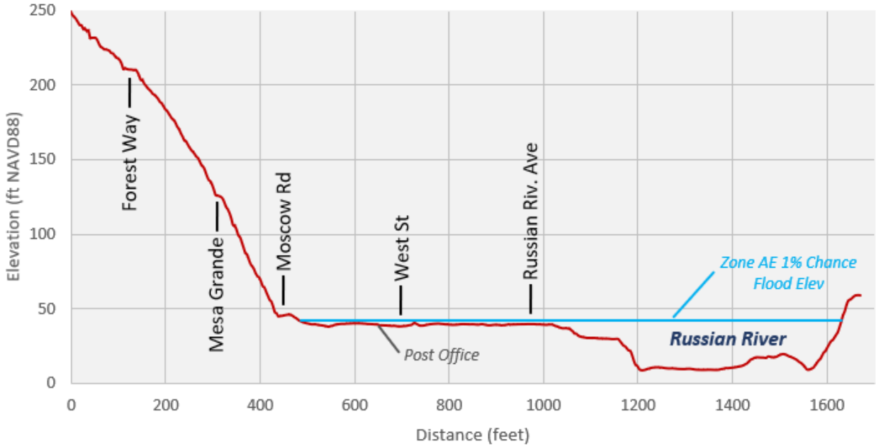
Figure 2-2: Ground Surface Profile Through Villa Grande, to the Russian River
