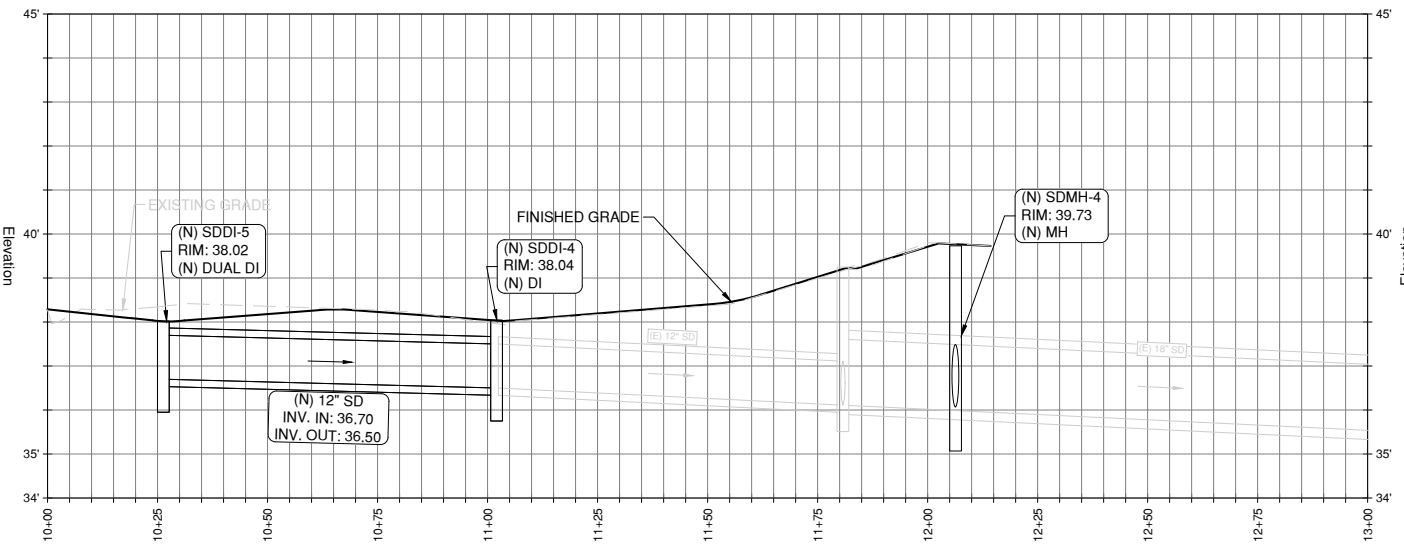
5TH STREET STORM SYSTEM IMPROVEMENT PROFILE
