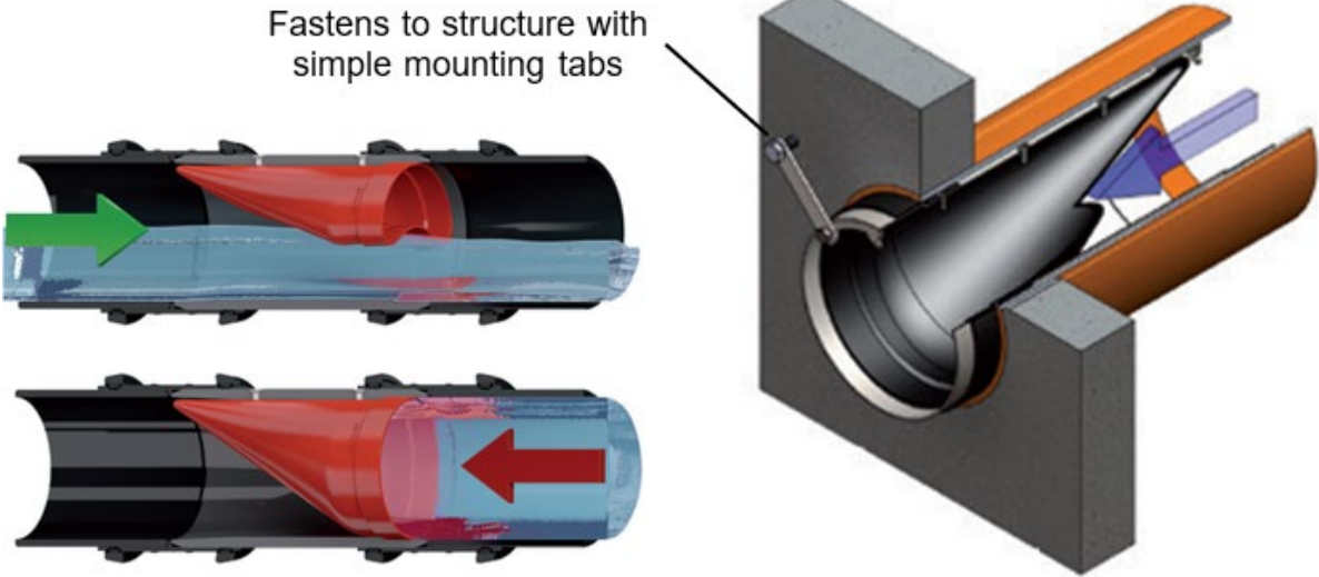
Figure 5-12: Inline Check Valve Operation (Left) and Installation in Existing Structure (Right)
