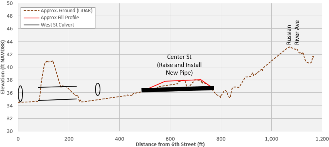
Figure 5-20: Alternative C-1 Plan (Top) and Approximate Profile (Bottom)
