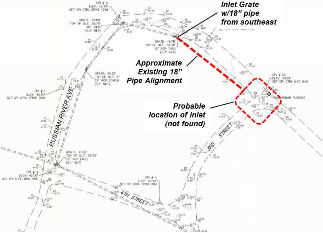
Figure 5-17: Surveyed System Around 3 rd Street Annotated with Probable Missing Inlet Location.
