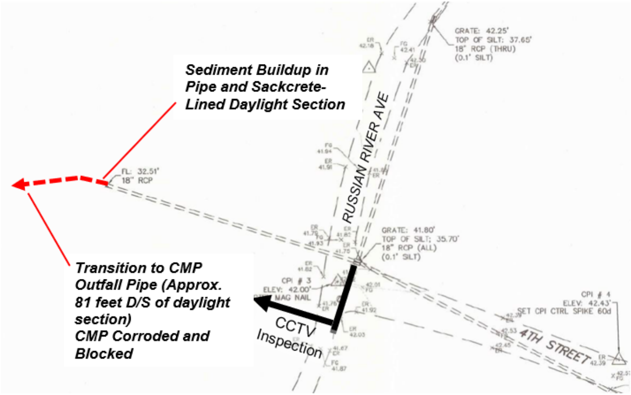
Figure 5-25: 4 th Street Outfall System
