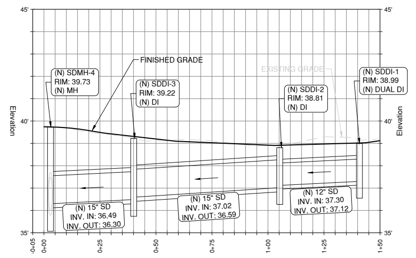
WEST STREET STORM SYSTEM IMPROVEMENT PROFILE
