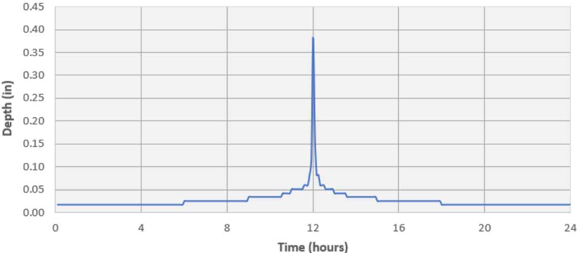
Figure 4-2: 24-hour, 10-year Storm for Villa Grande
