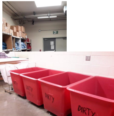
Dirty Laundry Carts- Top of cart 39 inches Bottom of cart- 9 inches off of floor Push force of 32.5 lbs.
