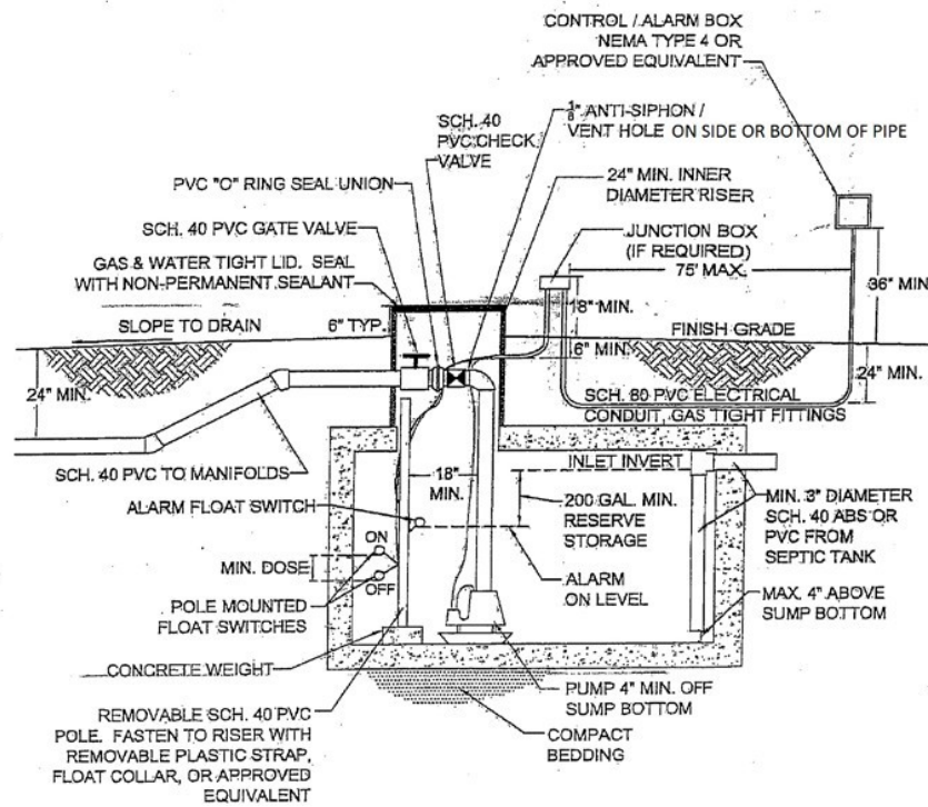
SUMP DETAIL (NOT TO SCALE)
